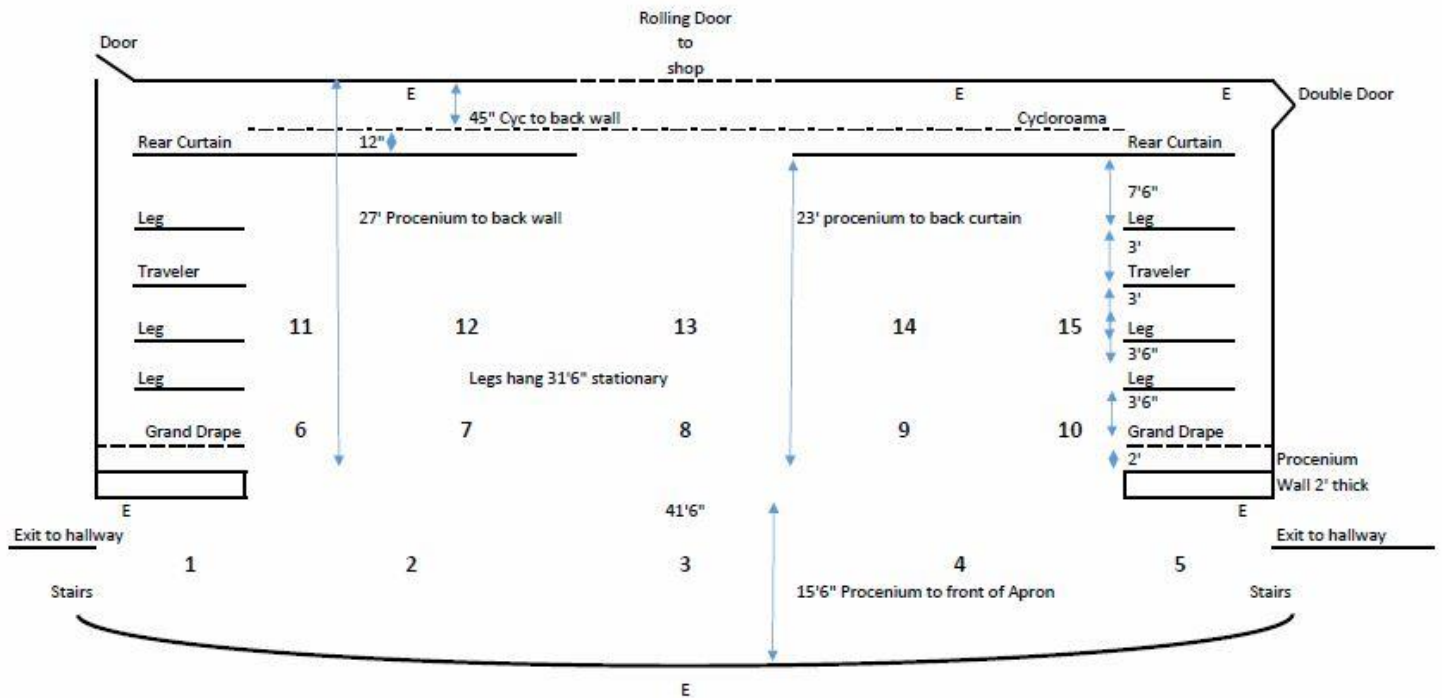
Central High School Fine Arts Center Light Plot and Dimensions
